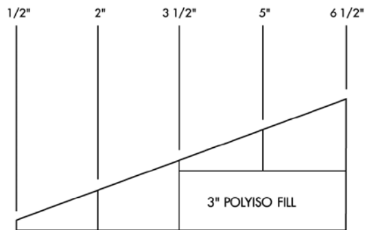
TYPICAL CROSS-SECTION OF 3/8" SLOPE P7
